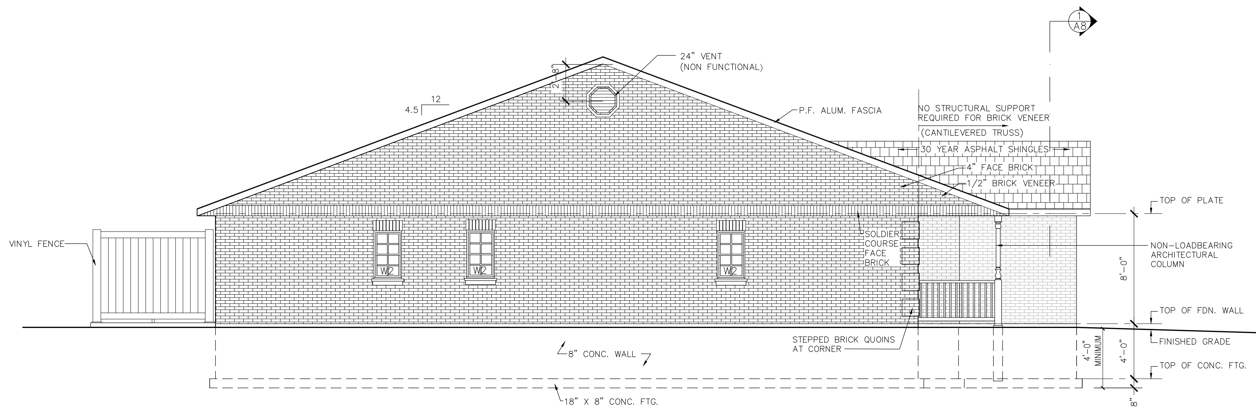
2 SIDE (EAST) ELEVATION A-6 SCALE: 1/4"=1'-0"
