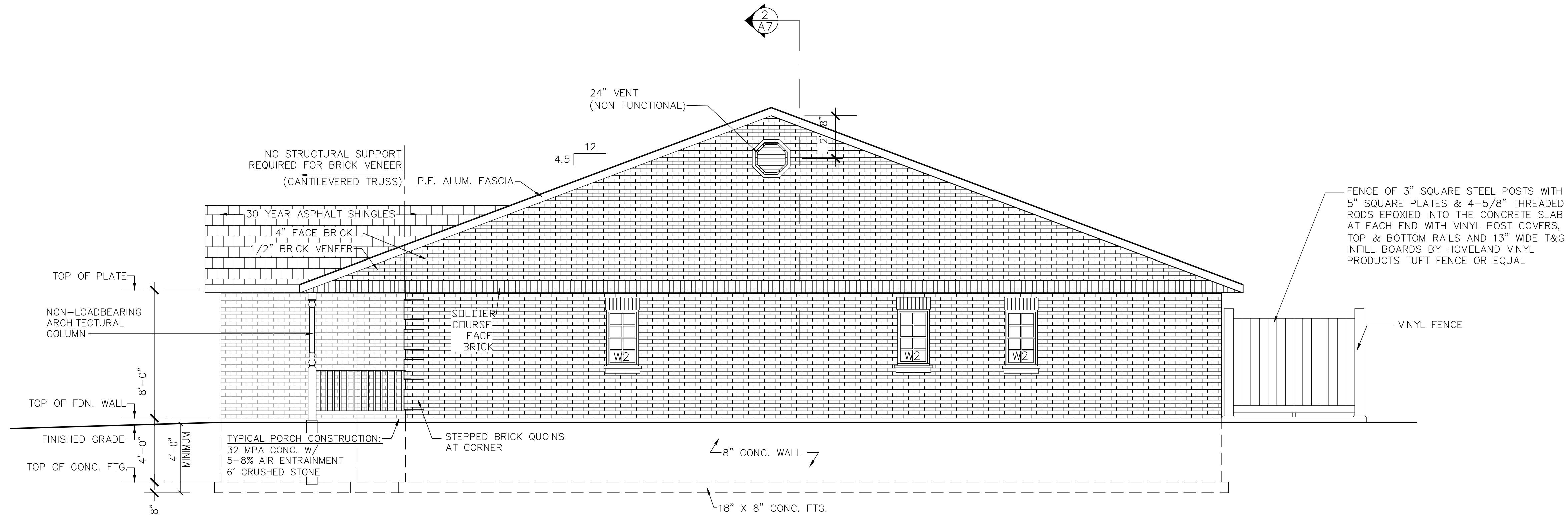
1 SIDE (WEST) ELEVATION A-6 SCALE: 1/4"=1'-0"
